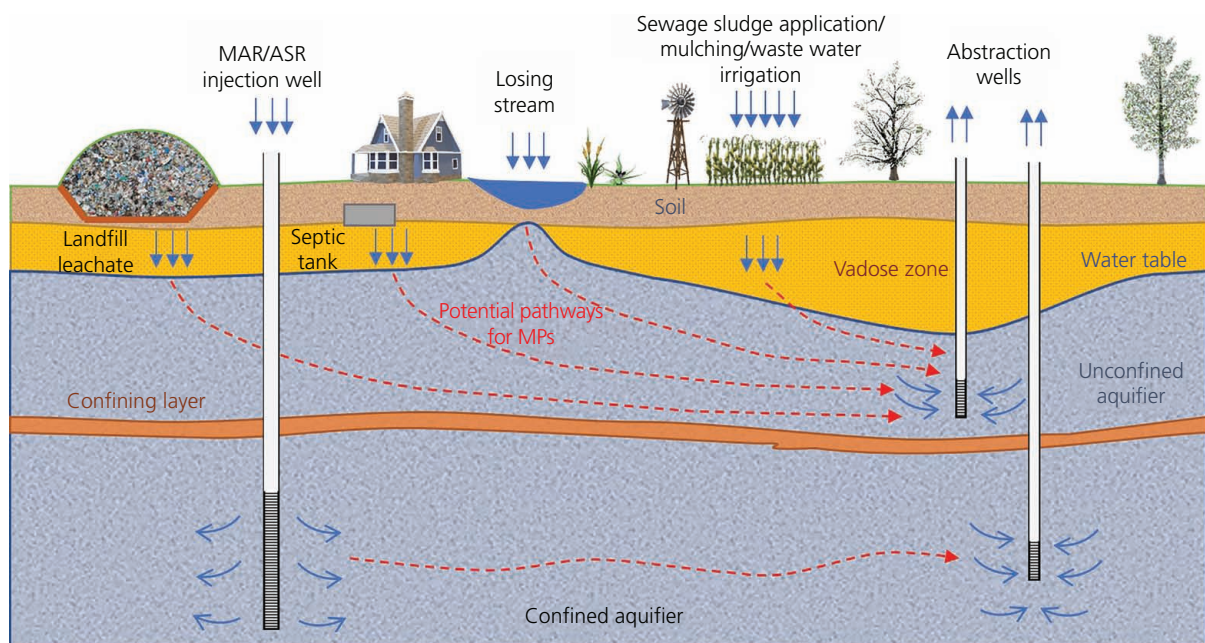
Figure 2. Schematic representation of possible pathways for MPs to enter and be transported through groundwater. ASR, aquifer storage and recovery; MAR, managed aquifer recharge
