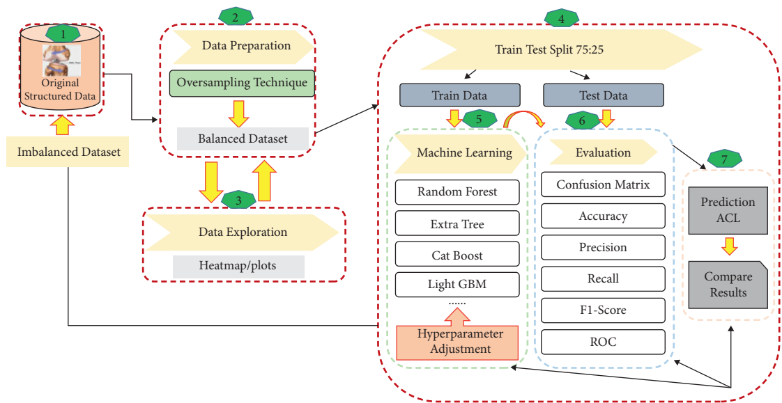
FIGURE 4: The proposed framework of our approach.
