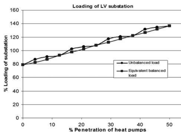
Fig. 5 Loading of LV substations with increasing penetration of heat pumps
