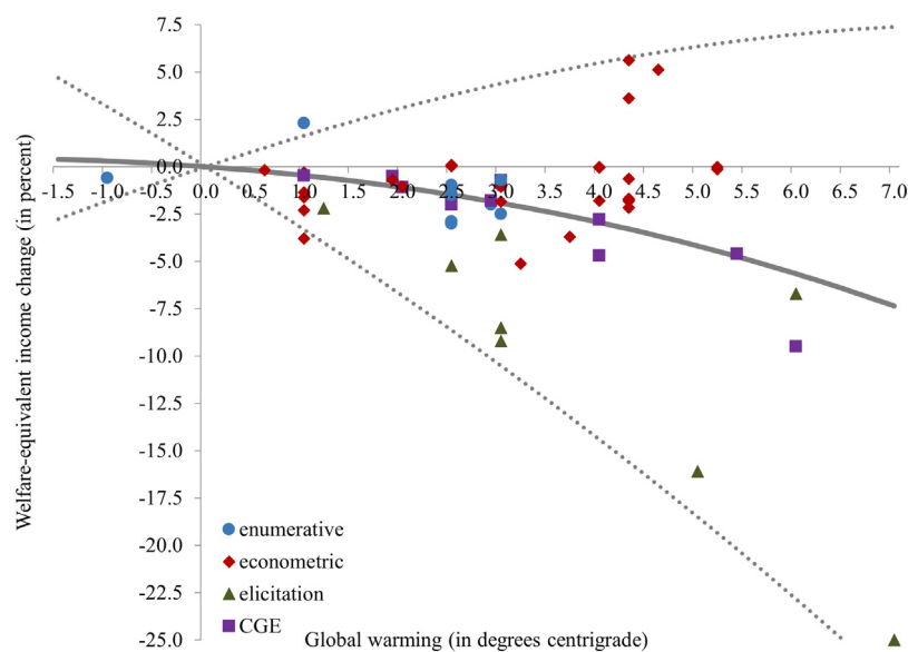
Fig. 1. The impact of climate change since pre-industrial times on global welfare according to comparative static studies.
