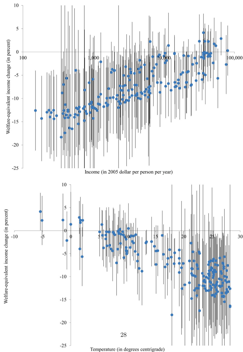
Fig. 5. The economic impact of climate change for a 2.5 °C warming relative to pre-industrial times for countries as a function of their income (top panel) and temperature (bottom panel).
