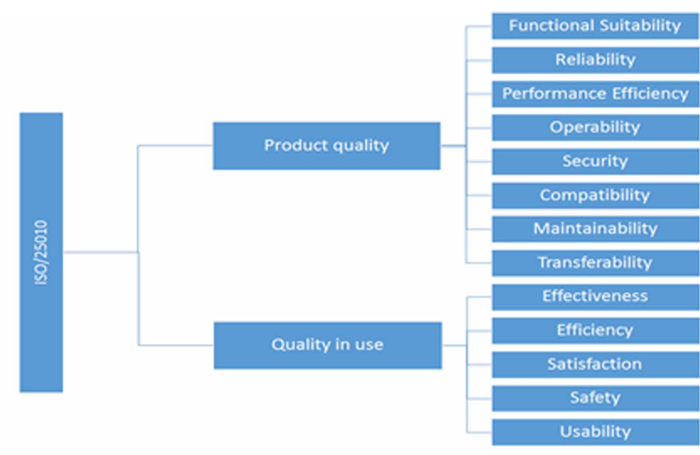
Figure 6. ISO/IEC 25010 (ISO/IEC 25010:2011)
