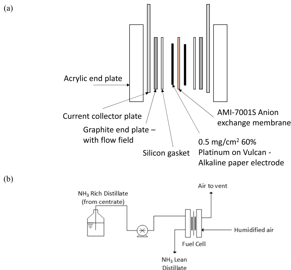
Fig. 2. Schematic of the direct ammonia fuel cell experimental set-up: (a) breakdown of the direct ammonia fuel cell and (b) diagram of the experimental set-up.
