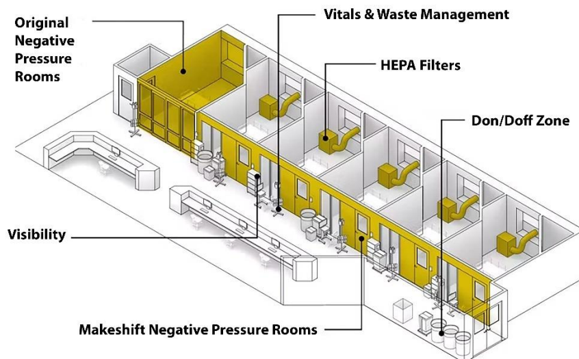
Figure 7. Alterations made to Mount Sinai Hospital's Guggenheim Pavilion rooms ( MASS Design Group, 2020 )
